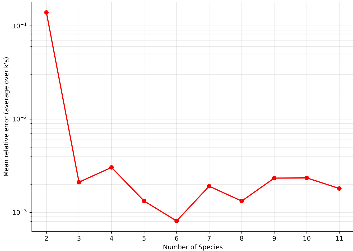
50, 50 — Mean relative error vs number of species
